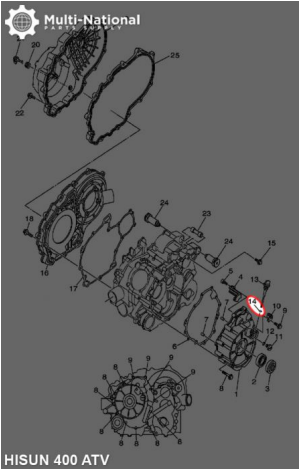
HISUN 400 ATV
